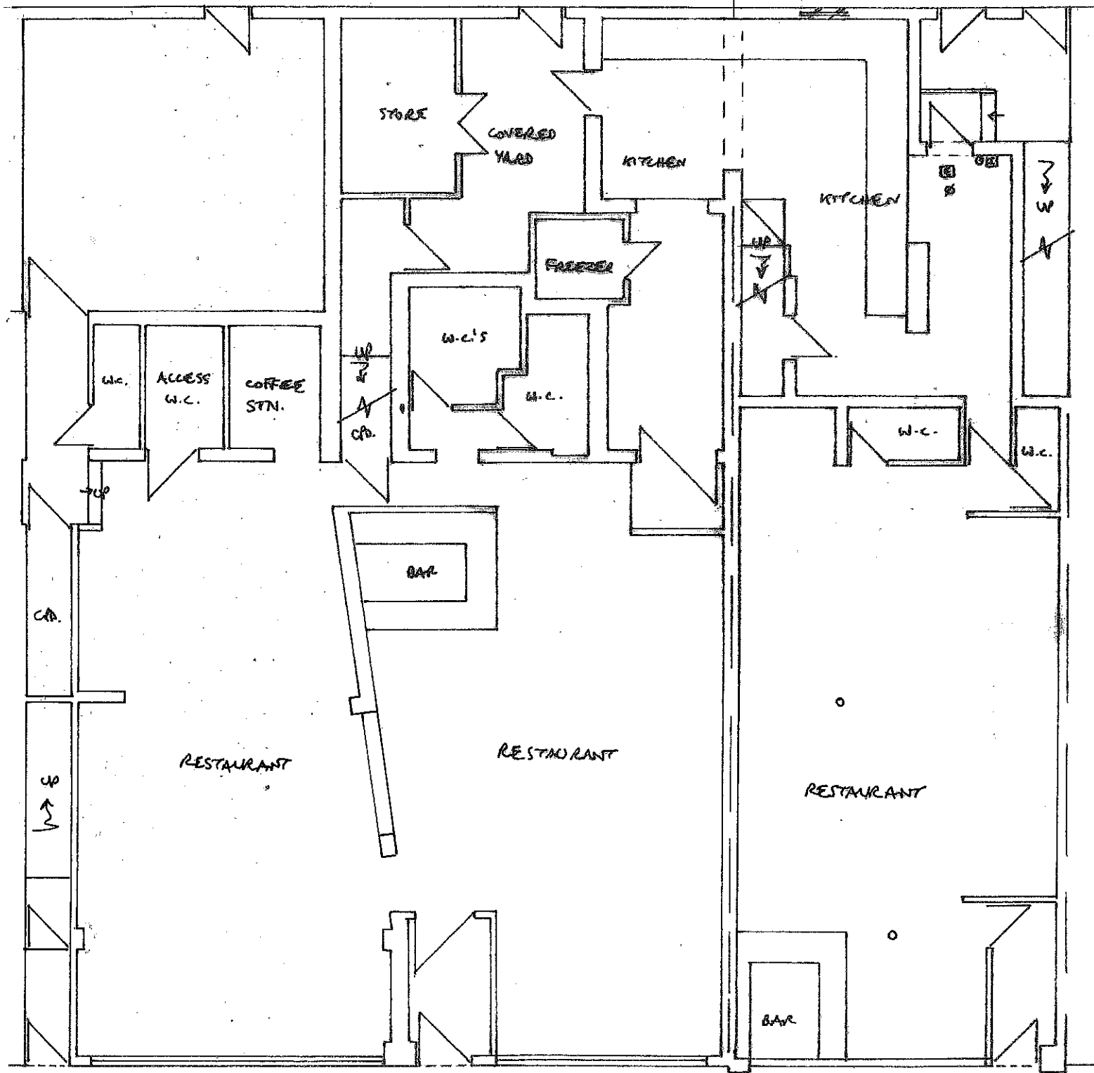
EXISTING PLAN 1:100
